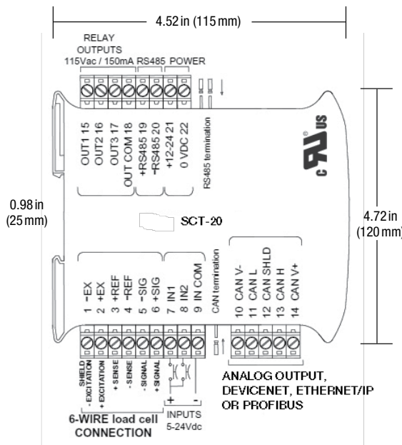
Dimensions: 0.98 x 4.52 x 4.72 in (25 x 115 x 120mm)
